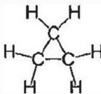
cyclopropane
