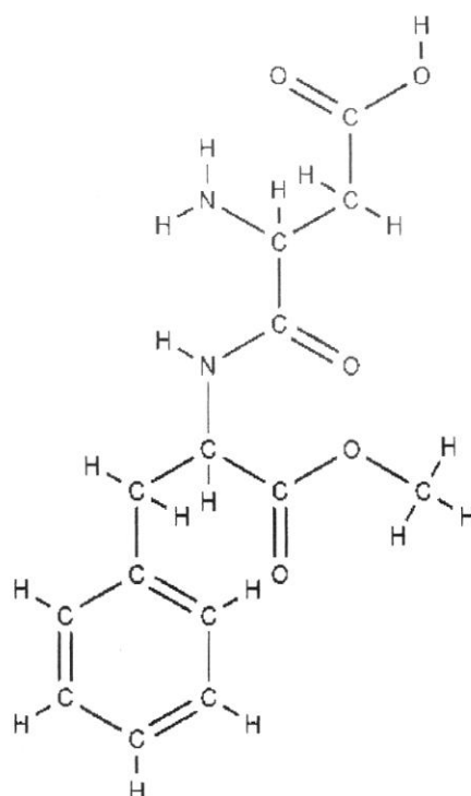
full structural formula of aspartame
