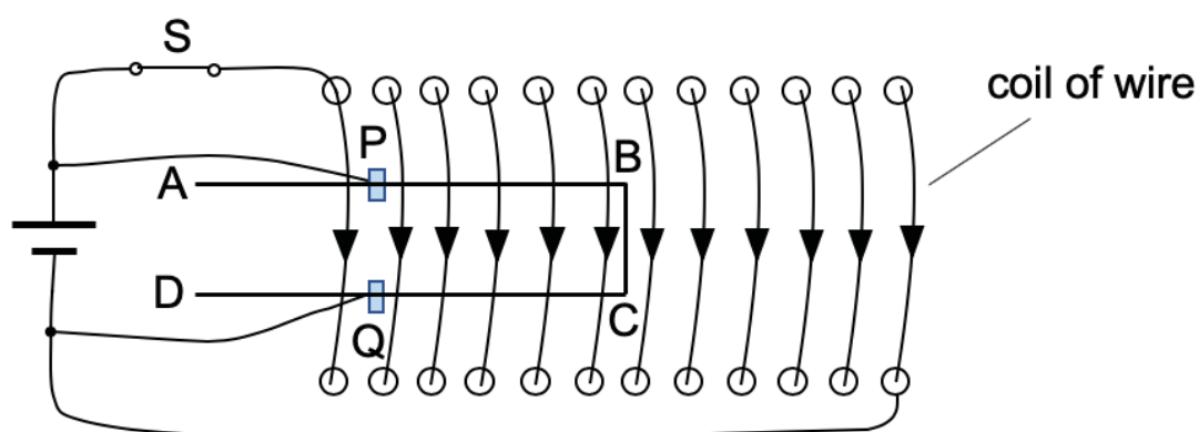
top view of set-up
